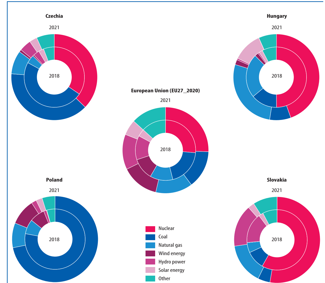
Distribution of net electricity generation, by energy source
