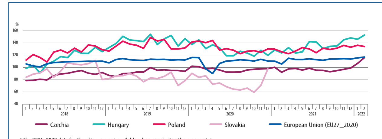
Volume index of civil engineering construction* (seasonally and calendar adjusted data, 2015=100%)
